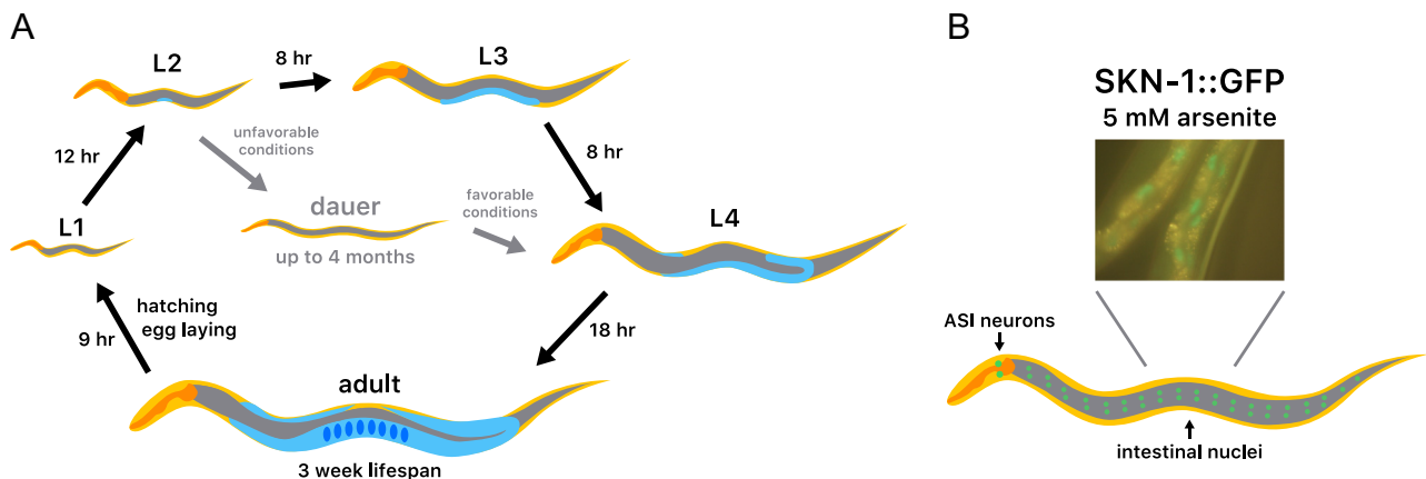
Fig. 2. Analysis of SKN-1 expression in vivo. (A) C. elegans life cycle stages. The hermaphrodite life cycle is shown [8]. The majority of C. elegans produced are hermaphrodites, which are typically studied in the laboratory. A small proportion of males are produced within each generation of approximately 300 animals. The pharynx, a pumping organ used for feeding, is shown in orange, the intestine in grey, the gonad in light blue, and embryos in dark blue. (B) SKN-1 protein expression. The expression pattern of a transgene that encodes the SKN-1b and SKN-1c isoforms is shown under stress conditions [7]. The SKN-1b isoform is expressed constitutively in the nuclei of the ASI neurons, and SKN-1c accumulates in intestinal nuclei in response to certain stresses [7,19].
